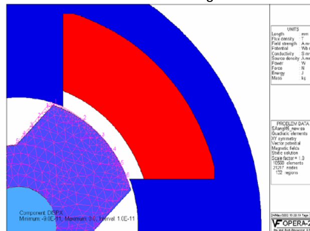
Deformation in rotor, shown as a displaced mesh
