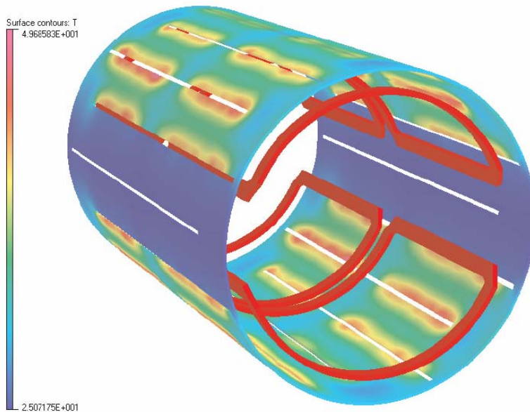
Temperature distribution in eddy current shield
