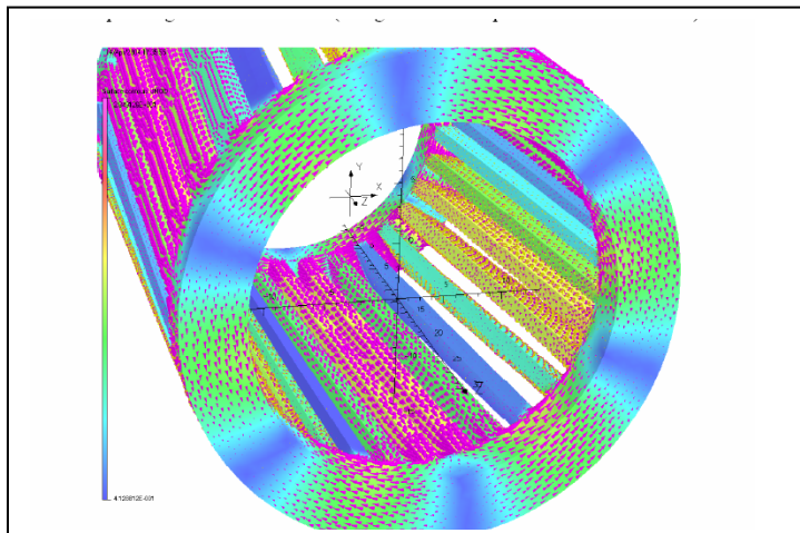
Rotor cage currents
