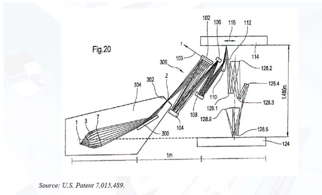
Collector and illuminator of EUV system.
